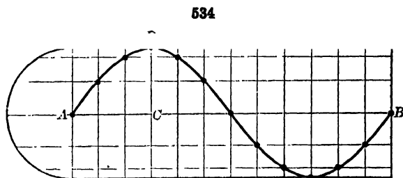
Harmonic Curve
